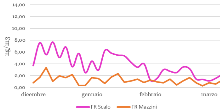
Benzo(a)pirene - 2025
