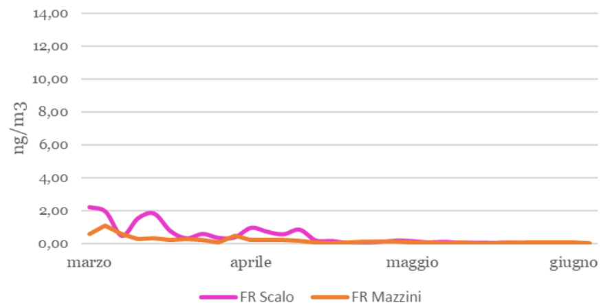
Benzo(a)pirene - 2025
