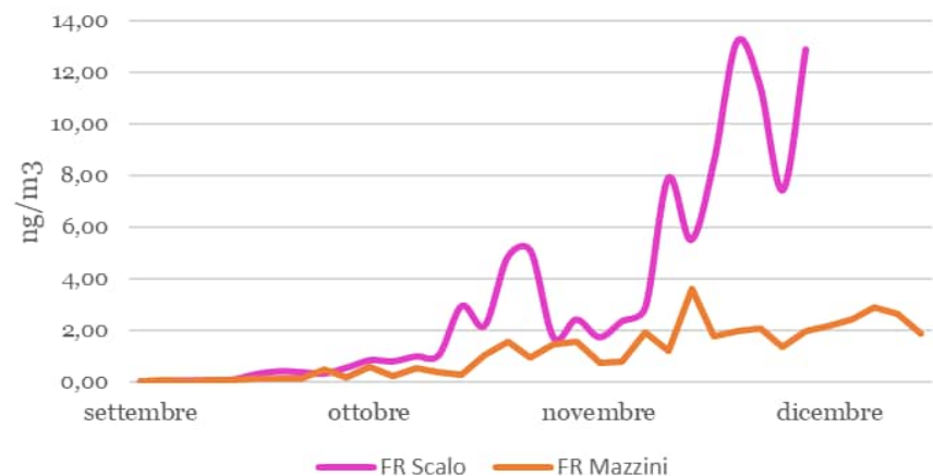
Benzo(a)pirene - 2025
