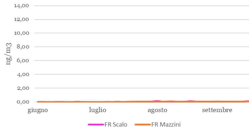
Benzo(a)pirene - 2025
